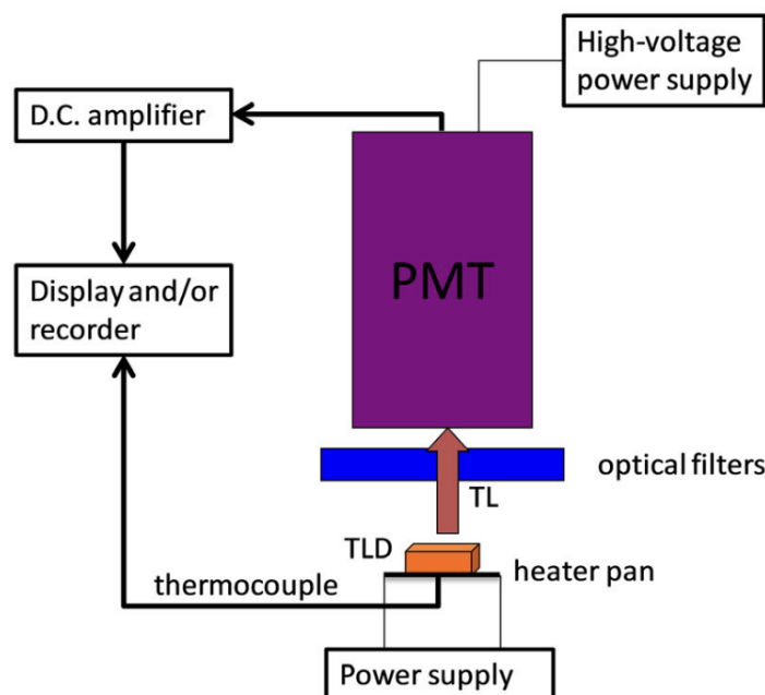
Figure 3: Schematic representation of a TLD reader system.
